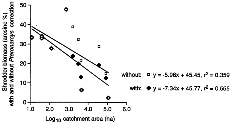
FIG. 2.—Shredder biomass based on assumption that all Pteronarcys spp. are detritivore-shredders (open squares) plotted against drainage basin area for various sites in the Little Tennessee River basin versus shredder biomass adjusted for proportion of Pteronarcys spp. guts containing detritus at various locations (dark diamonds)
