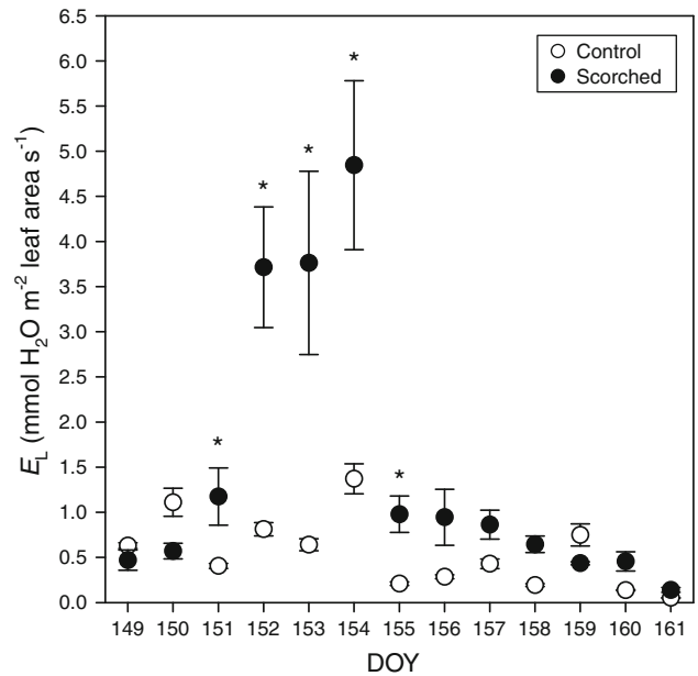
Fig. 2 Transpiration per unit leaf area ( E_L ) in scorch and control trees during the study period. Canopy scorching treatment was applied on day 150, and removed ca. 77% of the leaf area. Symbols represent the mean ( n = 3 ); error bars are one standard error. Asterisks indicate significant differences between scorch and control on those days at \alpha = 0.05 (one-tailed)
