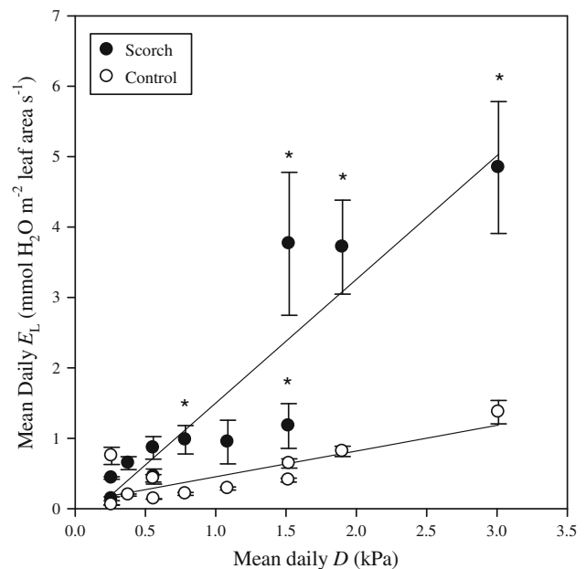
Fig. 3 Mean daytime transpiration per unit leaf area ( E_L ) in scorch ( R^2 = 0.83 ) and control ( R^2 = 0.64 ) trees during the treatment period (DOY 151–161) versus mean daytime air vapor pressure deficit ( D ). Lines differ significantly ( P = 0.047 ): control E_L = 0.42 D , scorched E_L = 1.19 D . Canopy scorching treatment was applied on day 150, and removed ca. 77% of the leaf area. Symbols represent the mean ( n = 3 ); error bars are one standard error. Asterisks indicate significant differences between scorch and control on those days at \alpha = 0.05 (one-tailed)
