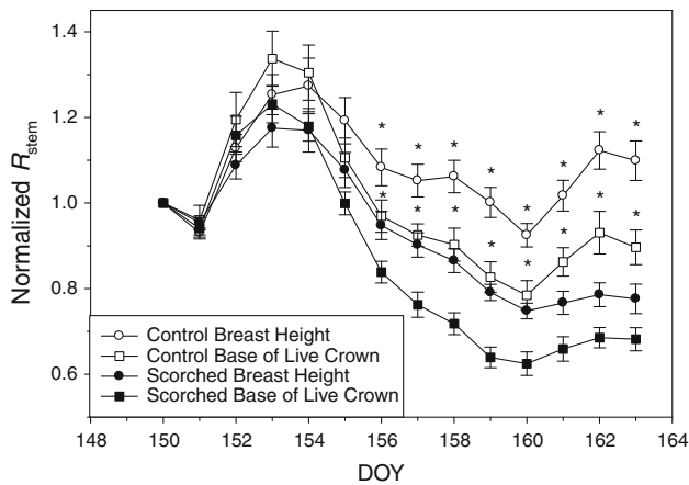
Fig. 4 Mean daily stem CO 2 efflux ( R_{\text{stem}} ; \mu\text{mol m}^{-2} \text{s}^{-1} ) normalized to day of year (DOY) 150 before scorching for chambers at breast height (BH) and base of live crown (BLC). Symbols represent the mean (BH, n = 8 , BLC, n = 4 ); error bars are one standard error. Asterisks indicate significant differences between treatments in both stem positions at \alpha = 0.05
