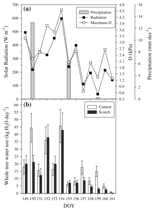
Fig. 1 Mean daytime air vapor pressure deficit ( D ), total precipitation ( P ), and mean daytime solar radiation ( a ), and whole tree water use in scorch and control trees ( b ) during the study period. Canopy scorching treatment was applied on day 150, and removed ca. 77% of the leaf area. Vertical bars in lower panel represent the mean of replicate trees ( n = 8 ); one standard error also shown
