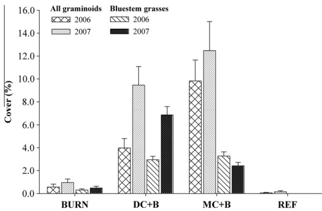
Fig. 6. Grass cover on the restoration treatments (burn only [BURN]; dry, cut + burn [DC + B]; sub-mesic, cut + burn [MC + B], and reference [REF] and the first two growing seasons (2006, 2007) after treatments.
