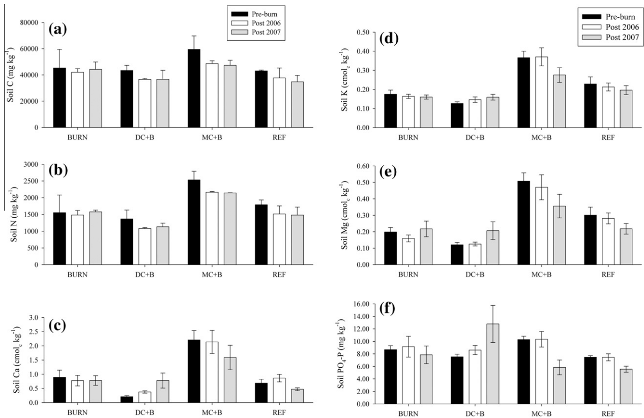
Fig. 2. Soil chemistry at 0–10 cm soil depth for the prescribed burn treatments (burn only [BURN]; dry, cut + burn [DC + B]; sub-mesic, cut + burn [MC + B], and reference [REF]) before (2005) and after restoration treatments (2006 and 2007): (a) total carbon ( \text{mg kg}^{-1} ), (b) total nitrogen ( \text{mg kg}^{-1} ), (c) exchangeable calcium, Ca ( \text{cmol}_c \text{kg}^{-1} ); (d) exchangeable potassium, K ( \text{cmol}_c \text{kg}^{-1} ); (e) exchangeable magnesium, Mg ( \text{cmol}_c \text{kg}^{-1} ); and (f) extractable ortho-phosphate, \text{PO}_4\text{-P} concentrations ( \text{mg kg}^{-1} ).
