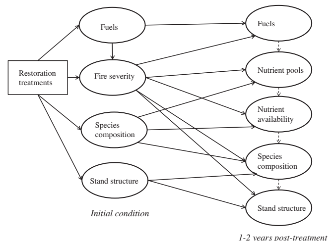
Fig. 1. Conceptual path model.
