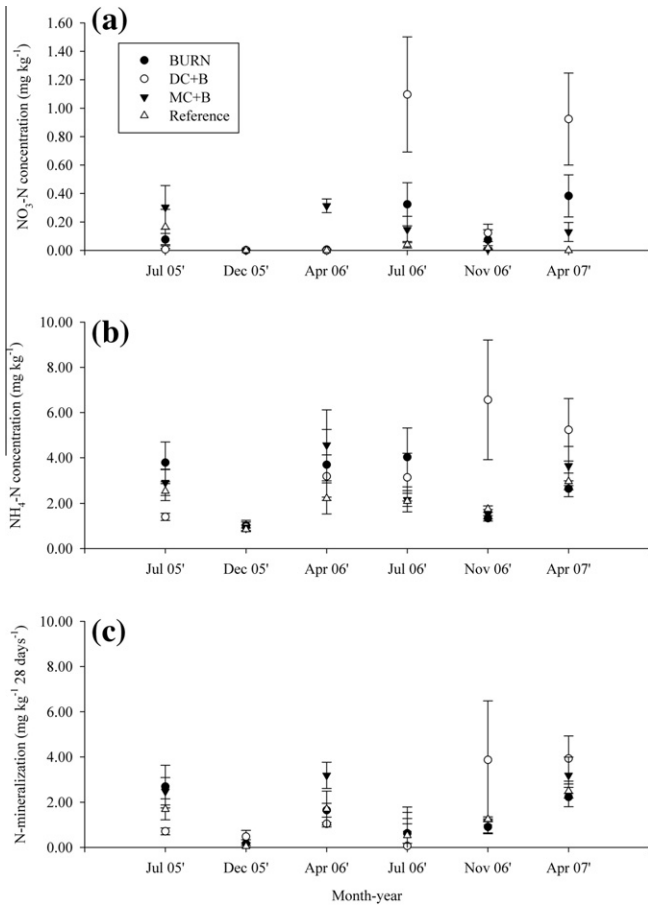
Fig. 3. Available soil nitrogen: (a) nitrate-nitrogen ( \text{NO}_3\text{-N} ) and (b) ammonium-nitrogen ( \text{NH}_4\text{-N} ) concentrations ( \text{mg kg}^{-1} ) and (c) N-mineralization ( \text{mg kg}^{-1} 28 \text{ days}^{-1} ) for the restoration treatments (burn only [BURN]; dry, cut + burn [DC + B]; sub-mesic, cut + burn [MC + B], and reference [REF]) before (2005) and after treatments (2006 and 2007):
