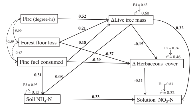
Fig. 8. Final structural equation models with standardized path coefficients for soil solution nitrate-nitrogen at 0–30 cm soil depth for March–April 2007 ( \text{NO}_3\text{-N}_{2007} ) and herbaceous layer cover change between preburn-2005 and postburn-2007 ( \chi^2 = 9.348 , df = 7 , P = 0.229 , and model goodness of fit CFI = 0.970, NFI = 0.905, and NNFI = 0.909). Variables used in model are described in Fig. 7 , and soil \text{NH}_4 = soil ammonium-nitrogen concentration in 2007; solution \text{NO}_3 = soil solution \text{NO}_3 at 30 cm soil depth in 2007; and \Delta herbaceous cover = herbaceous layer cover 2005 – herbaceous layer cover 2007.
