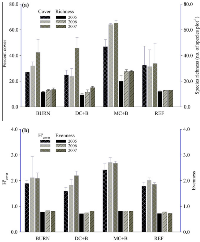
Fig. 5. Herbaceous layer response for the restoration treatments (burn only [BURN]; dry, cut + burn [DC + B]; sub-mesic, cut + burn [MC + B], and reference [REF] before (2005) and the first two growing seasons (2006, 2007) after treatments: (a) percent cover and species richness and (b) diversity based on percent cover ( H'_{cover} , Shannon's index) and evenness of species distribution.
