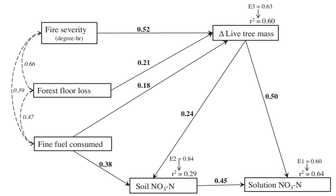
Fig. 7. Final structural equation models with standardized path coefficients for soil solution nitrate-nitrogen at 0–30 cm soil depth for June–August 2006 ( \text{NO}_3\text{-N}_{2006} ) ( \chi^2 = 8.49 , df = 5 , P = 0.128 , and model goodness of fit CFI = 0.961, NFI = 0.919, and NNFI = 0.882). Variables used in the model are: fire severity as estimated by degree-hr; forest floor loss = preburn \text{O}_i + \text{O}_e + \text{O}_a forest floor – postburn \text{O}_i + \text{O}_e + \text{O}_a forest floor; fine fuel consumed = preburn fine fuel (down small wood <7.5 cm diameter) – postburn fine fuel; \Delta live tree = preburn live tree biomass – postburn live tree biomass; soil \text{NO}_3 = soil nitrate-nitrogen concentration in 2006; and solution \text{NO}_3 = soil solution \text{NO}_3 at 30 cm soil depth in 2006.
