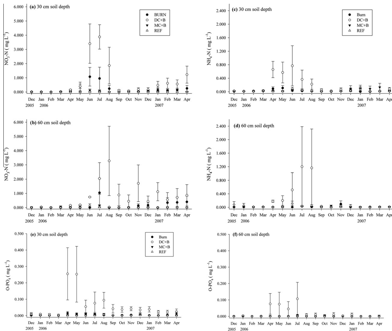
Fig. 4. Soil solution chemistry for the restoration treatments (burn only [BURN]; dry, cut + burn (DC + B); sub-mesic, cut + burn [MC + B], and reference (REF) four months before (December 2005– March 2006) and thirteen months (April 2006 – April 2007) after treatments: nitrate-nitrogen, \text{NO}_3\text{-N} (a) 30 cm soil depth, (b) 60 cm soil depth; ammonium-nitrogen, \text{NH}_4\text{-N} (c) 30 cm soil depth, (d) 60 cm soil depth; and ortho-phosphate, \text{PO}_4\text{-P} concentrations (e) 30 cm soil depth, (f) 60 cm soil depth.
