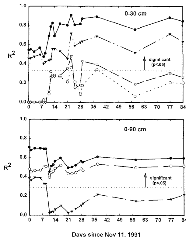
Fig. 3. Squared partial correlations for physiographic variables vs. soil moisture content during the measurement period. Physiographic variables shown are: topographic index ( \nabla ), soil storage index ( \circ ), and organic matter index ( \nabla ). Also shown are adjusted r^2 values for multiple regressions of physiographic variables on soil moisture ( \bullet ); only those variables that were significant in partial F tests ( p < .05 ) were included.
