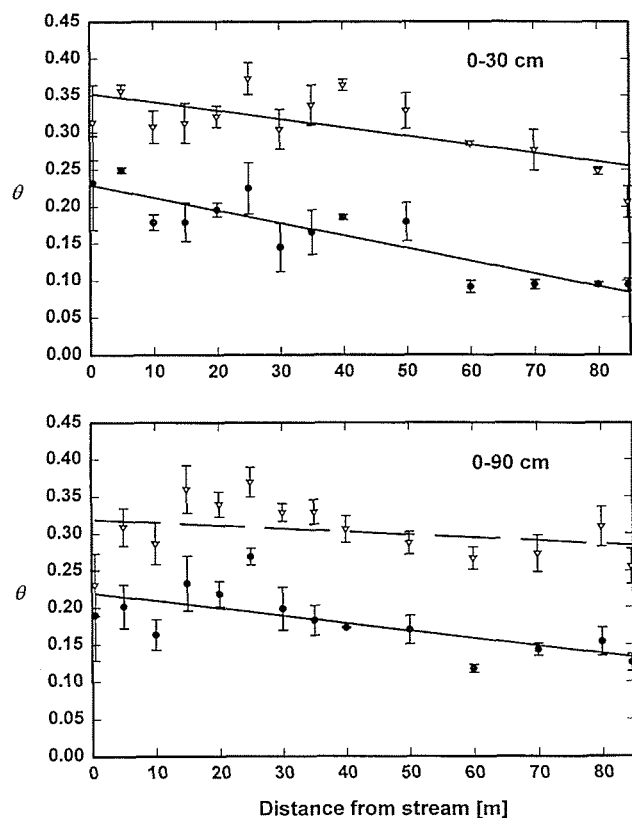
Fig. 2. Soil moisture response ranges: from drought (11 November, 1991; \bullet ) through 24.3 cm precipitation recharge (2 December, 1991; \nabla ). Each point is a mean of 3 measurements. Least squares regressions of soil moisture content on distance along hillslope in the shallow layer showed significant ( p < .05 ) gradients before and after recharge. Regressions in the deeper layer showed a significant gradient during drought, but not after recharge.
