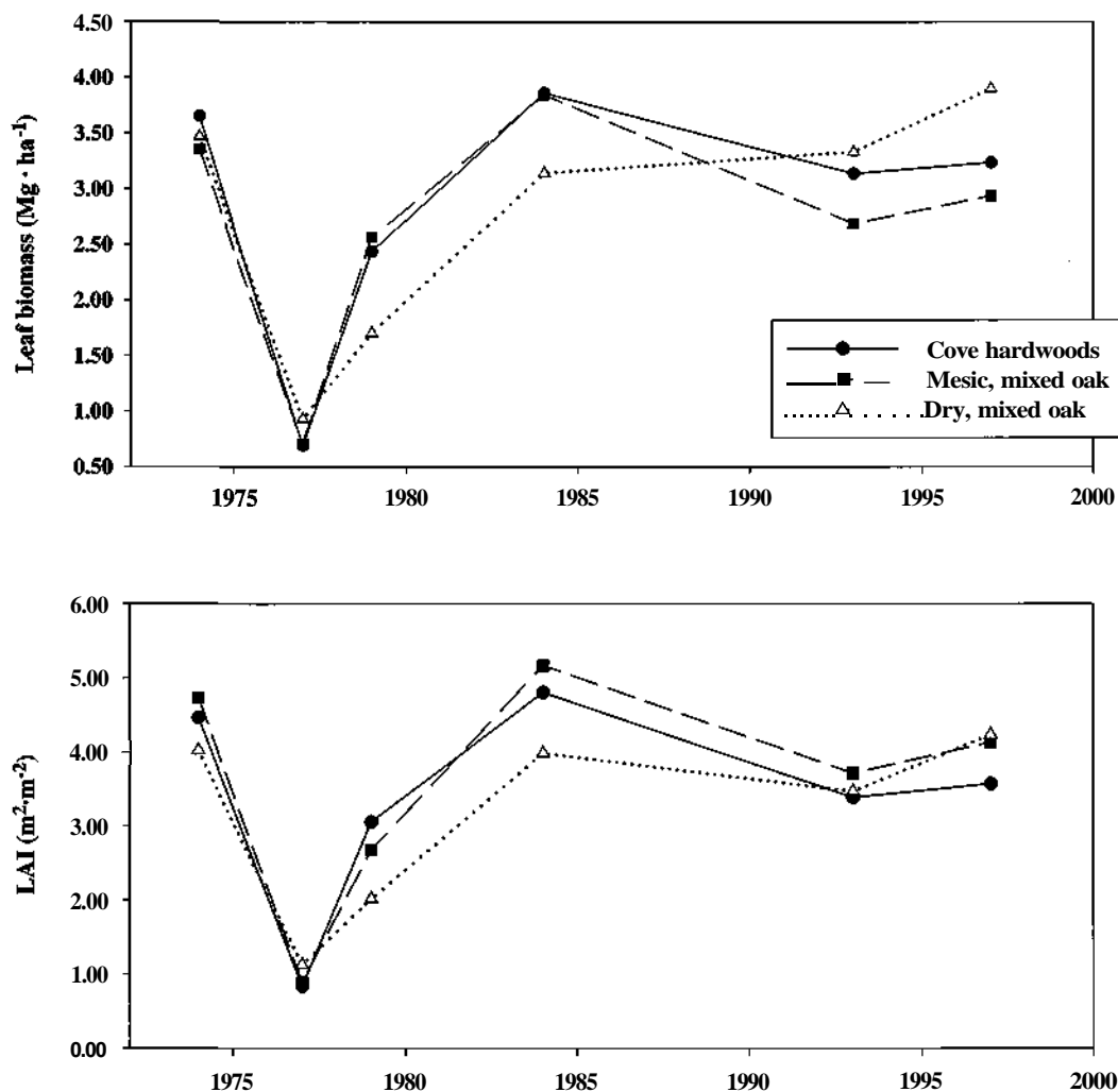
Fig. 2. Leaf biomass and leaf area index (LAI) for the three community types (cove hardwoods; mesic, mixed oak; and dry, mixed oak) before cutting (1974) and after cutting (1977, 1979, 1984, 1993, and 1997) for WS7, Coweeta Basin, western North Carolina.
