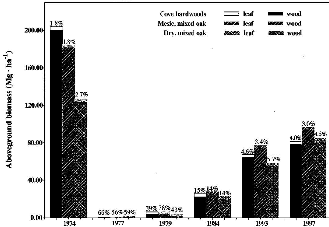
Fig. 1. Aboveground live biomass of woody species ( \geq 1.0 cm diameter base of stem) and herbaceous layer species (herbaceous + woody species < 0.5 m height) for the three community types (cove hardwoods; mesic, mixed oak; and dry, mixed oak) before cutting (1974) and after cutting (1977, 1979, 1984, 1993, and 1997) for WS7, Coweeta Basin, western North Carolina. The herbaceous layer was not sampled in 1997. Values above bars are percent contribution of leaf tissue to total aboveground biomass.
